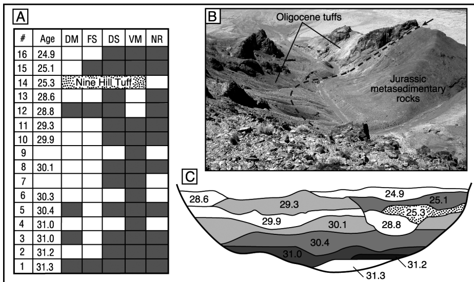
Figure 2. A: Shaded boxes indicate presence of tuff in paleovalley segment (see Fig. 3B for locations and abbreviation definitions; ages are in millions of years). B: Northern margin (dashed line) of paleovalley, Nightingale Range (looking west). C: Schematic paleovalley fill at Dogskin Mountain, with ages corresponding to individual tuffs.
